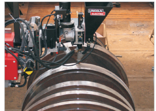
Hard-surfacing of turbines
