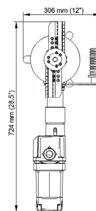
PRO-10 PB cu motor electric
